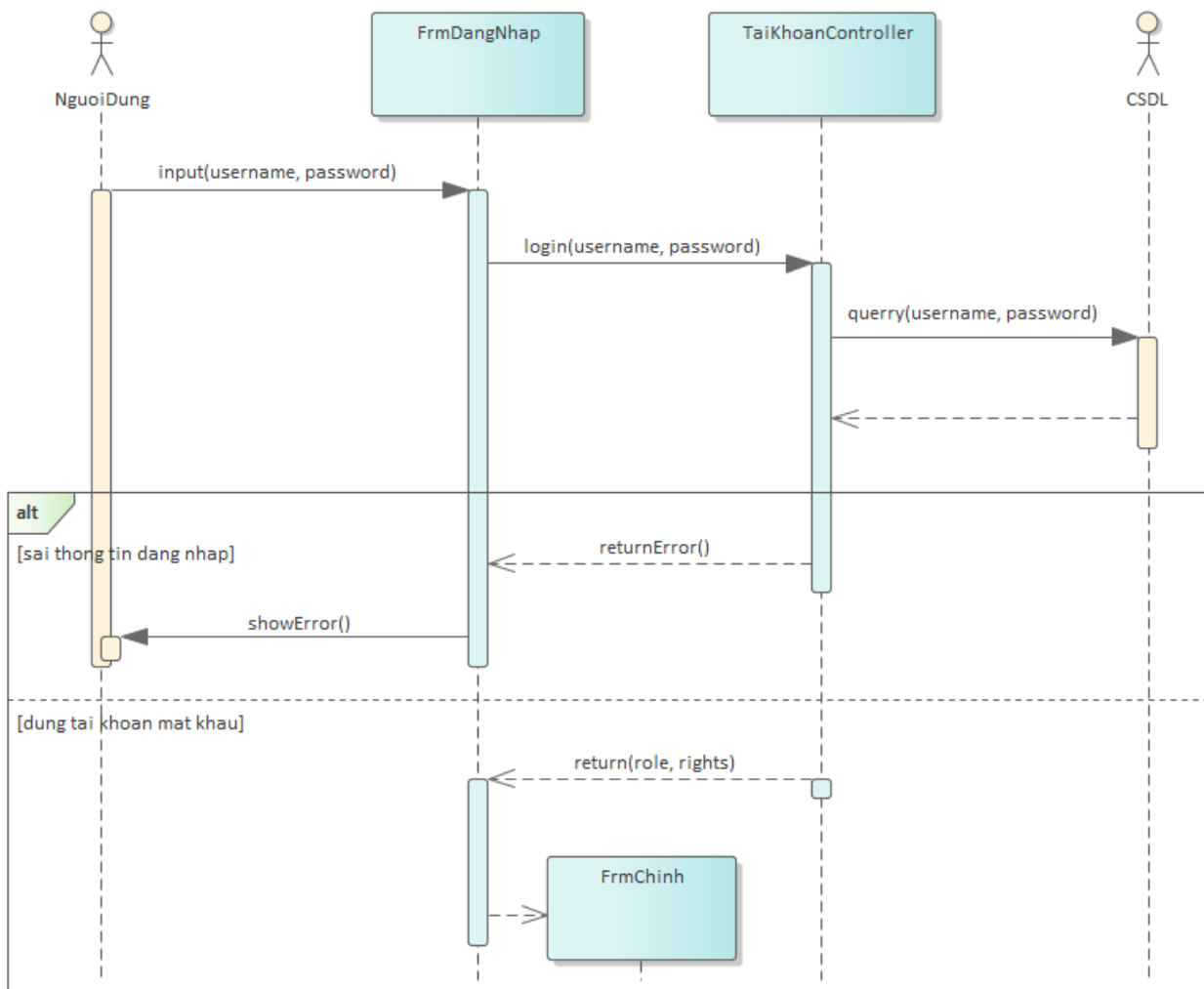
Figure 4: Dang nhap Sequence
