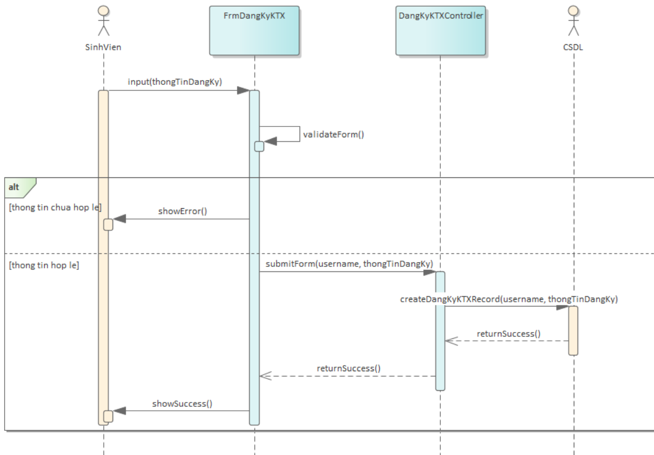
Figure 2: Dang ky KTX Sequence
