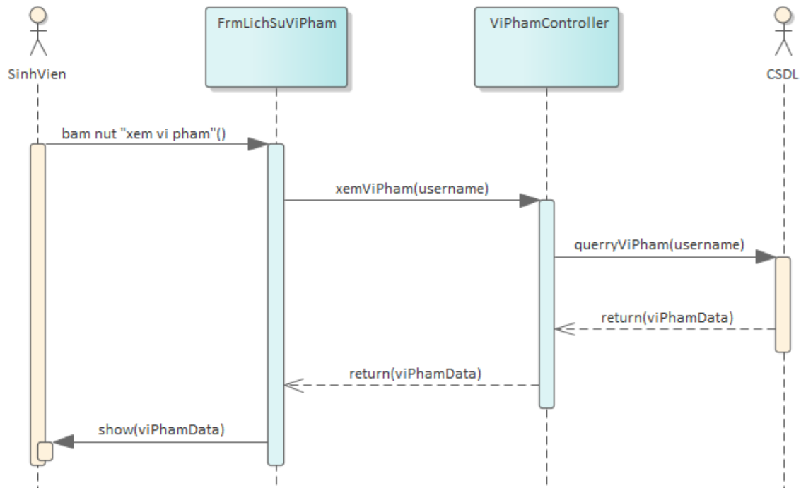
Figure 11: Xem lich su vi pham Sequence
