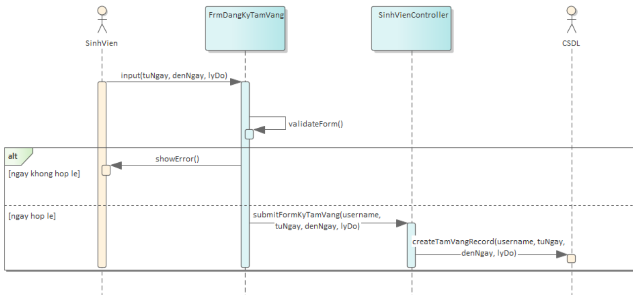
Figure 3: Dang ky tam vang Sequence
