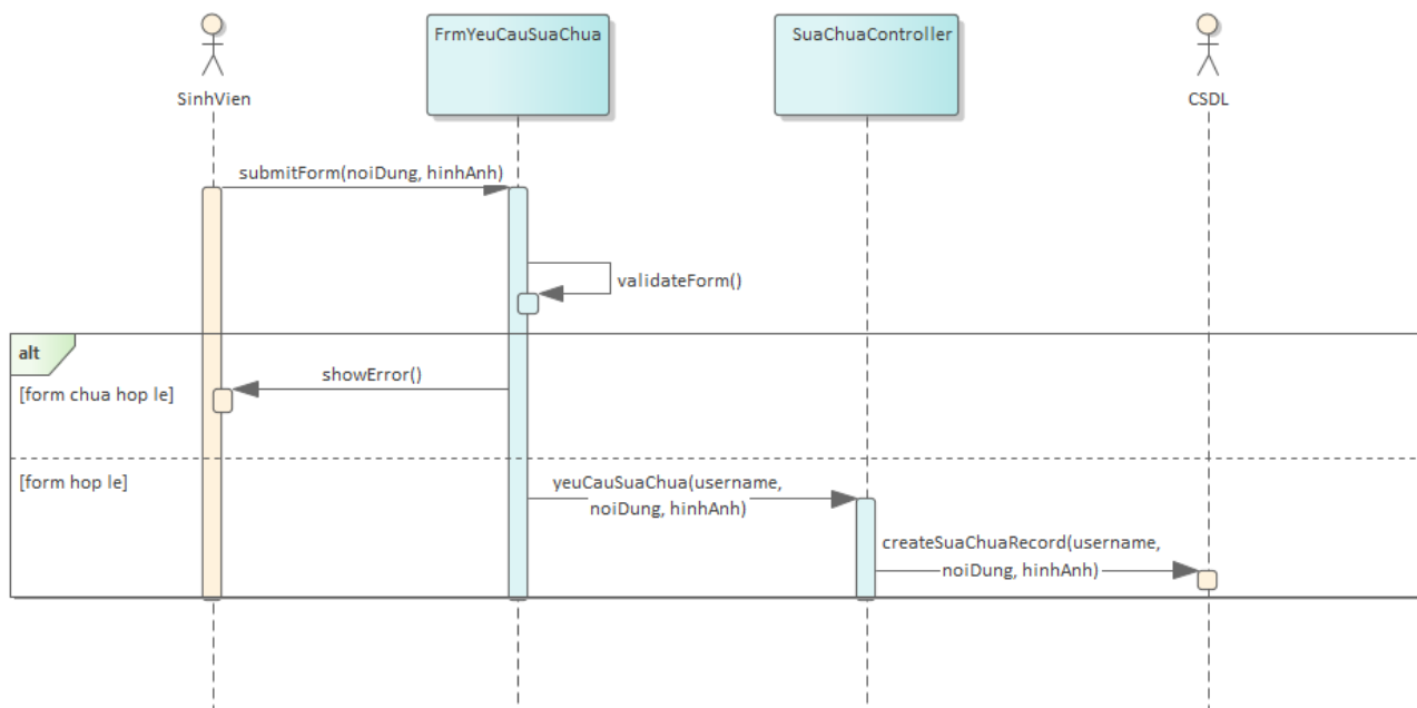
Figure 6: Gui yeu cau sua chua Sequence
