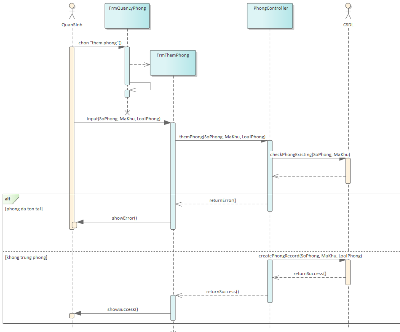
Figure 7: Them phong Sequence
