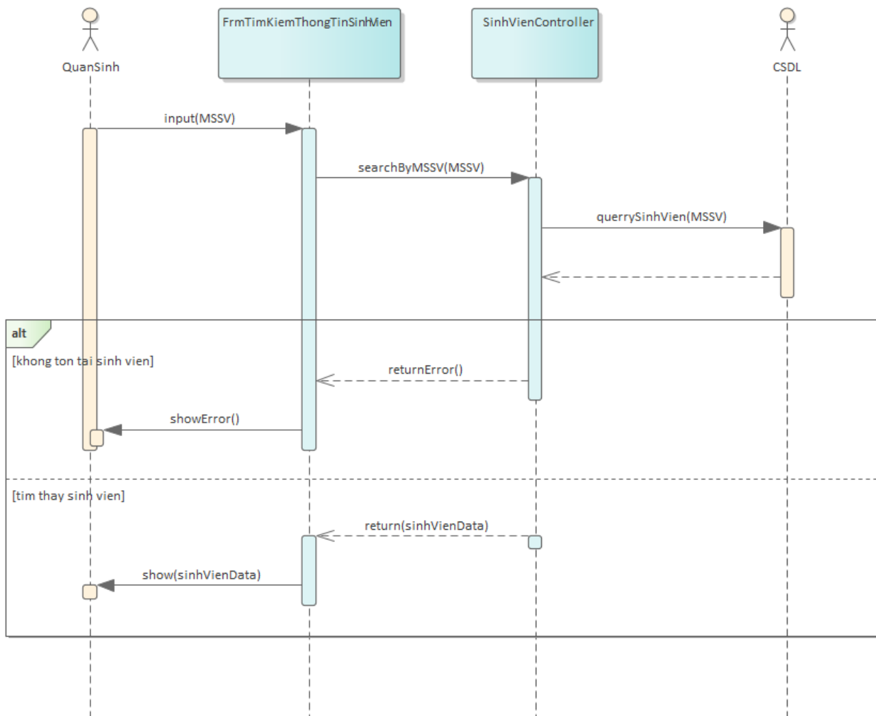
Figure 10: Timkiemthongtinsinhvien Sequence
