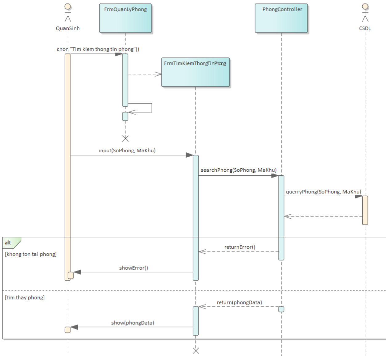
Figure 9: Timkiemthongtinphong Sequence
