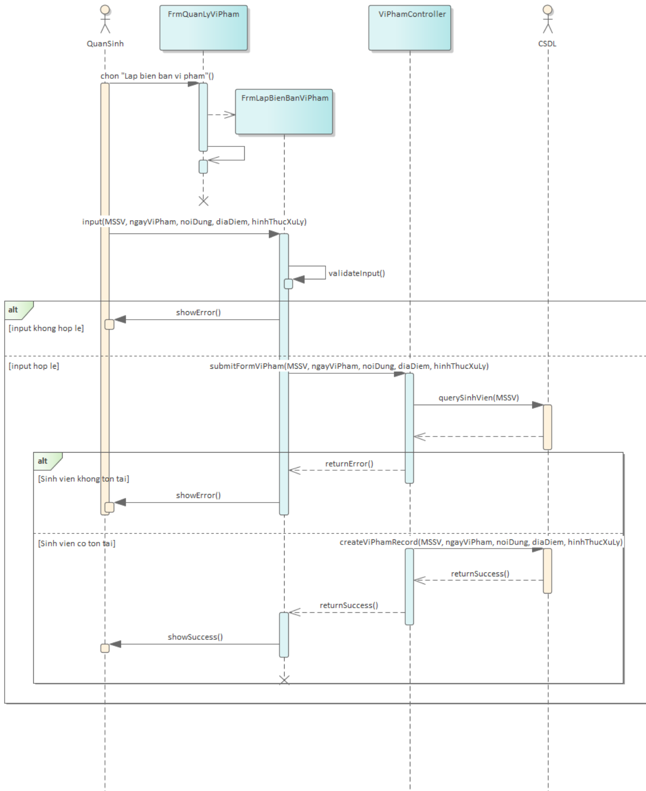
Figure 8: Lap bien ban vi pham Sequence
