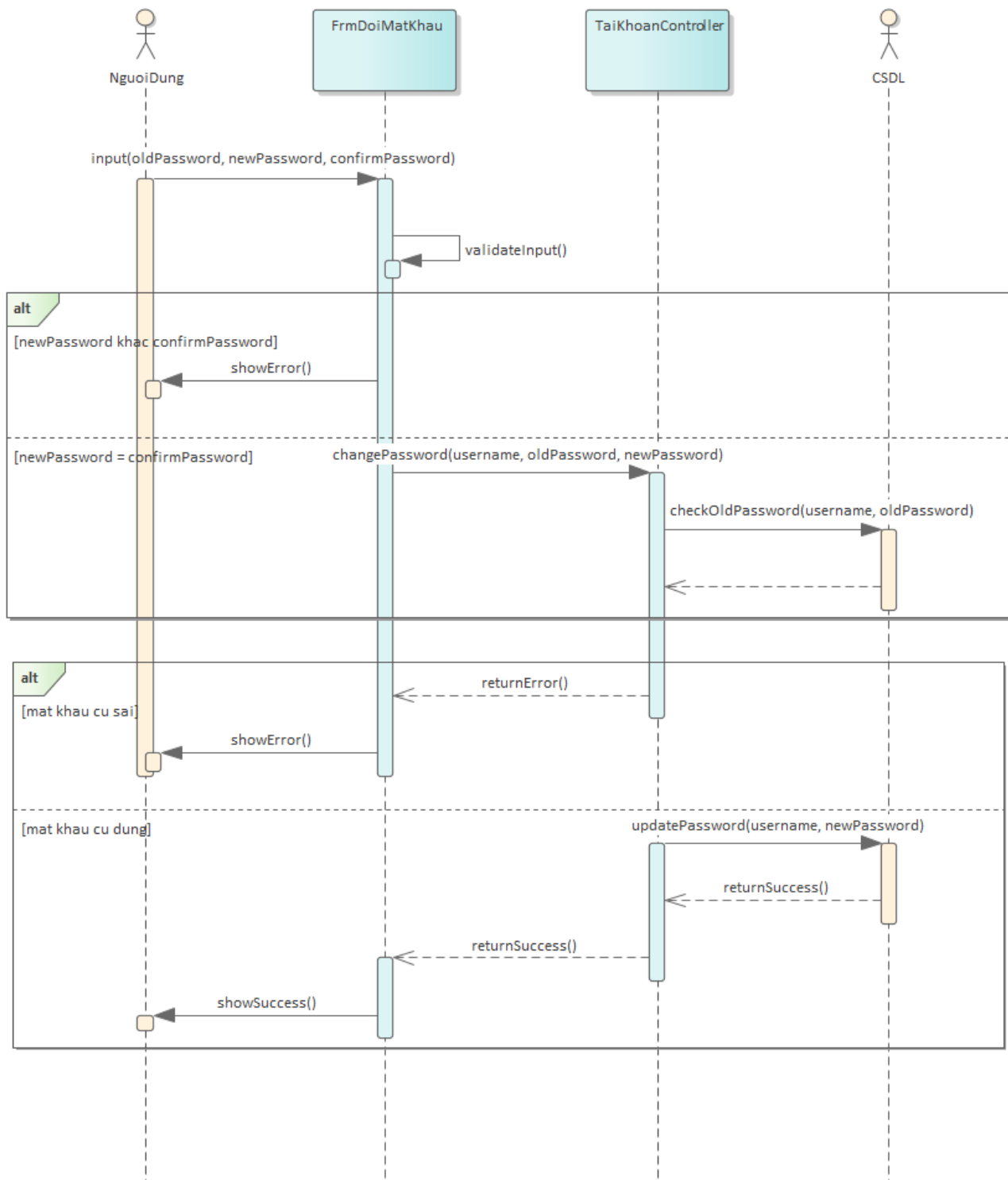
Figure 5: Doi mat khau Sequence
